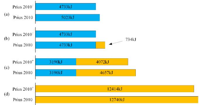
Figure 10 Energy analysis for different available battery energy
