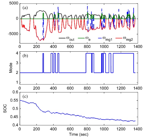
Figure 9 Component speed and Mode selection for Prius2010 +
