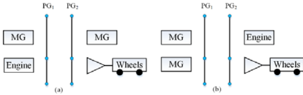
Figure 2. Two configuration types: engine and vehicle on the different PG (a) or same PG (b)
