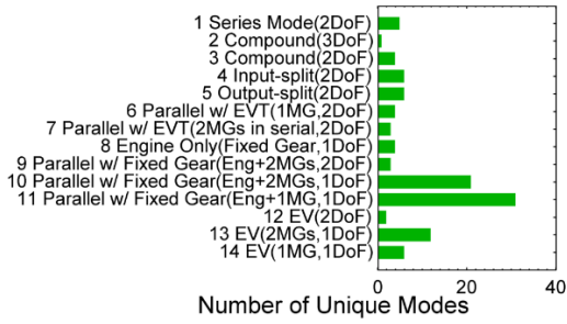
Figure 6. All feasible and non-redundant modes for the THS-II Configuration (used in Prius 2010)
