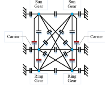
Figure 4. All 21 possible clutch locations for double PG system, the four highlighted in red are redundant and the one that ground the vehicle node is considered infeasible in this paper
