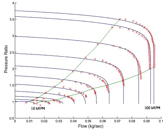
Figure 7 Compressor map
